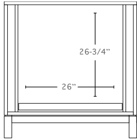
Amp Tray
