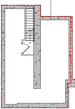
Lower Level
